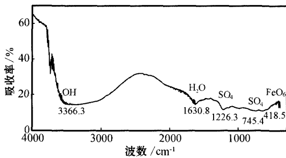
图3 施氏矿物红外光谱图 Fig. 3 FTIR spectra of synthetic schwertmannite
