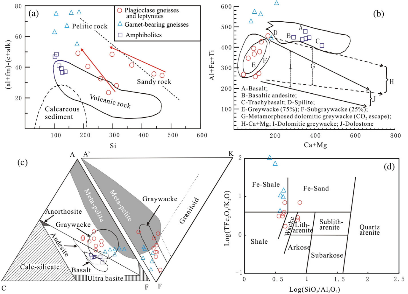
Fig. 8. Diagrams of (al + fm) - (c + alk) vs. Si (a), (Ca + Mg) vs. (Al + Ti + Fe) (b), ACF-A'KF (c) and \log(SiO_2/Al_2O_3) vs. \log(TFe_2O_3/K_2O) (d) discriminating the protoliths of metamorphic rocks. (a), (b), (c) and (d) are modified after Simonen (1953), Moine and de La Roche (1968), Winkler (1976), and Herron (1988), respectively.
