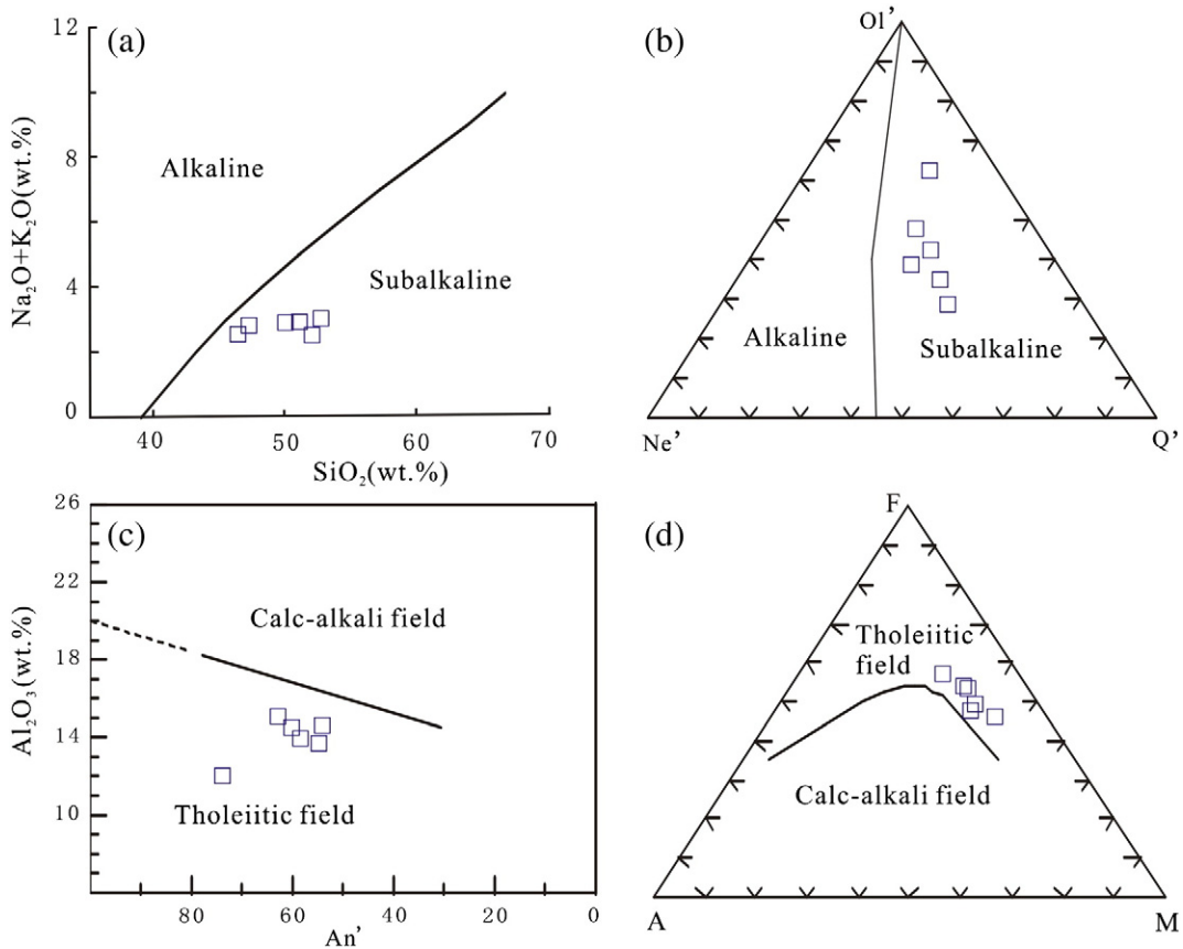
Fig. 12. Diagrams of SiO 2 vs. K 2 O + Na 2 O (a), Ol'-Ne'-Q' (b), An' vs. Al 2 O 3 (c) and AFM (d) dividing the basalts into different suites. All the diagrams are from Irvine and Baragar (1971). Ol', Ne', Q' and An' are calculated by using the cation norm, Ol' = Ol + 3/4Opx, Ne' = Ne + 3/5Ab, Q' = Q + 2/5Ab + 1/4Opx, An' = 100An/(An + Ab + 5/3Ne). F = FeO + 0.8998Fe 2 O 3 , A = K 2 O + Na 2 O, M = MgO, all in weight percent.
