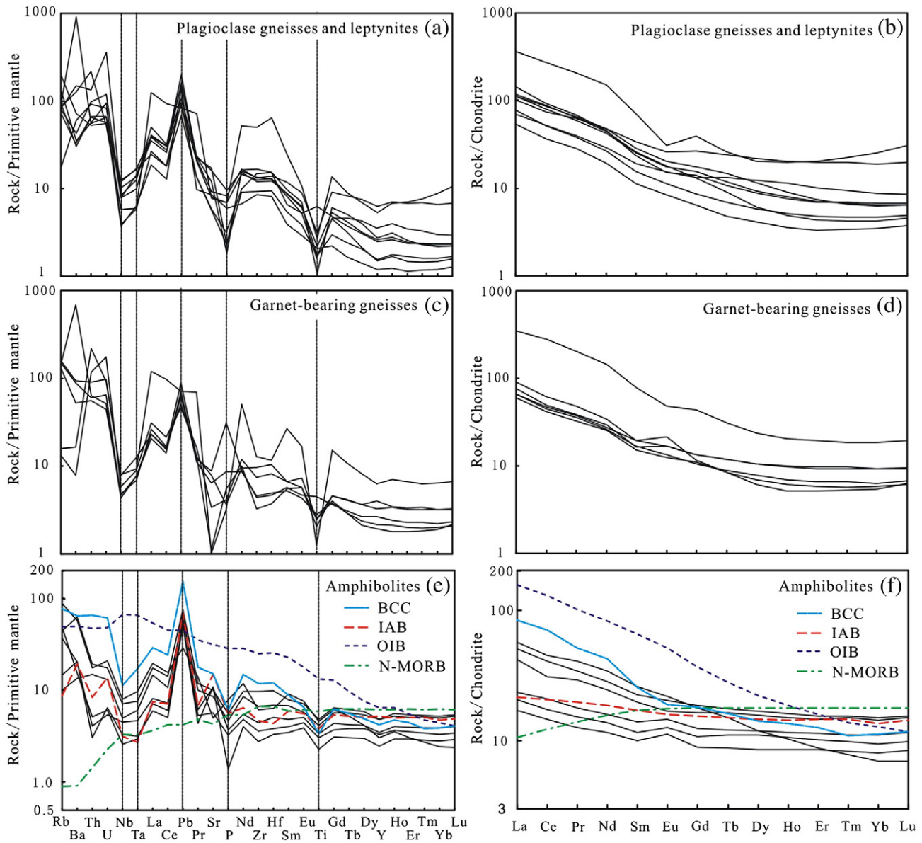
Fig. 6. Primitive Mantle (PM) normalized trace element diagrams and Chondrite-normalized REE patterns for the plagioclase gneisses (a, b), garnet-bearing gneisses (c, d) and amphibolites (e, f). Bulk continental crust (BCC), island arc basalts (IAB), ocean island basalts (OIB) and normal-type mid-ocean ridge basalts (N-MORB) are shown for comparison. The values of PM, Chondrite, OIB and N-MORB are from Sun and McDonough (1989). The IAB is from Takahashi et al. (2011), and the BCC is from Rudnick and Gao (2003).
