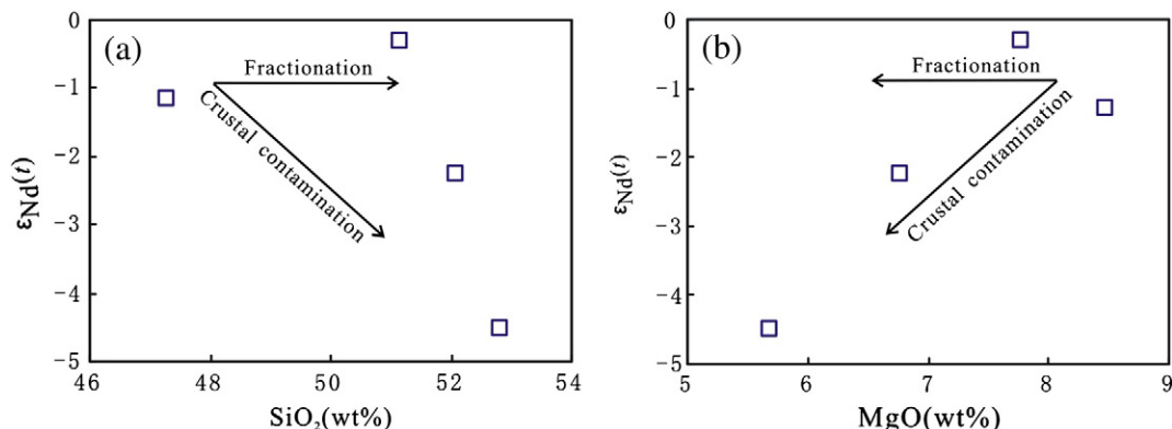
Fig. 14. Plots of \epsilon_{\text{Nd}}(t) vs. \text{SiO}_2 (a) and \epsilon_{\text{Nd}}(t) vs. MgO (b) for the meta-tholeiites from the Changyi BIF area.
