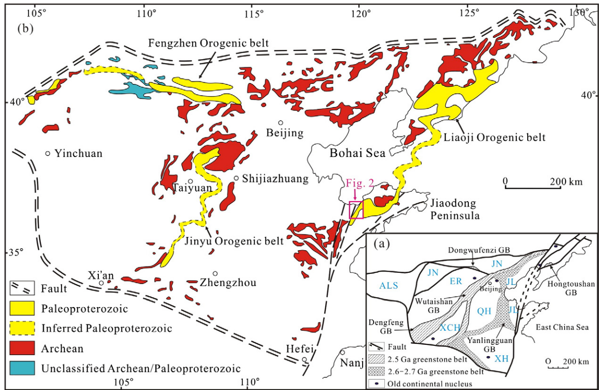
Fig. 1. (a) Sketch map of the NCC showing distribution of ancient nuclei, Archean micro-blocks and greenstone belts. (b) Distribution of Paleoproterozoic mobile belts of the North China Craton. Both (a) and (b) are modified after Zhai and Santosh (2011). JL: Jiaoliao Block; QH: Qianhuai Block; OR: Ordos Block; JN: Jining Block; XCH: Xuchang Block; XH: Xuhuai Block; ALS: Alashan Block; GB: greenstone belt.
