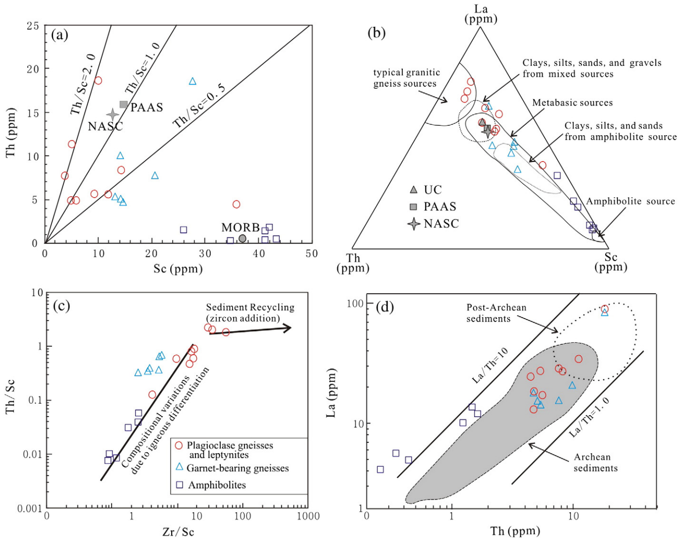
Fig. 9. Diagrams of Th vs. Sc (a), La-Th-Sc (b), Th/Sc vs. Zr/Sc (c) and La vs. Th (d) for discriminating the provenance of the meta-sedimentary rocks. Post-Archean Australian Shale (PAAS, McLennan, 1989), North American Shale Composite (NASC, Gromet et al., 1984) and upper continental crust (UC, Taylor and McLennan, 1985) are shown for comparison in (a) and (b). (b), (c) and (d) are after Cullers (1994), McLennan et al. (1993) and McLennan (1989), respectively.
