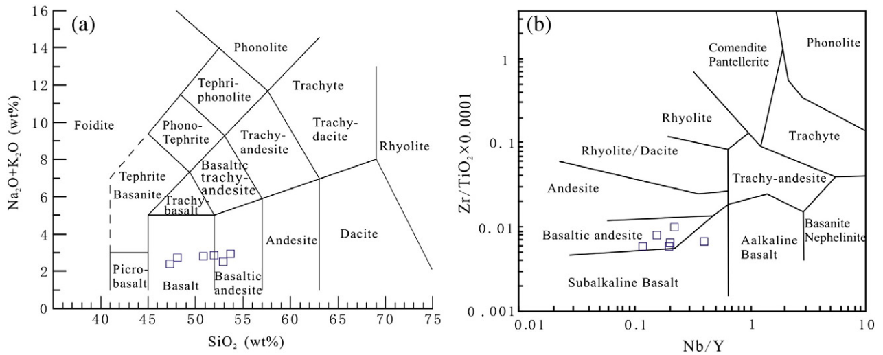
Fig. 11. Diagrams of (Na 2 O + K 2 O) vs. SiO 2 (TAS) (a) and Zr/TiO 2 vs. Nb/Y (b) for volcanic rocks nomenclature. (a) and (b) are after Le Bas et al. (1986) and Winchester and Floyd (1976), respectively.
