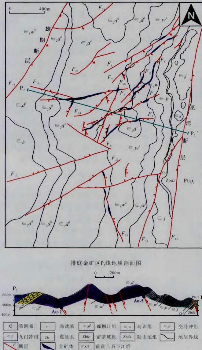
图2 排庭金矿床地质简图(据范二川,2010 修改) Fig.2 Geological sketch map of the Paiting gold deposit (modified after Fan, 2010)
