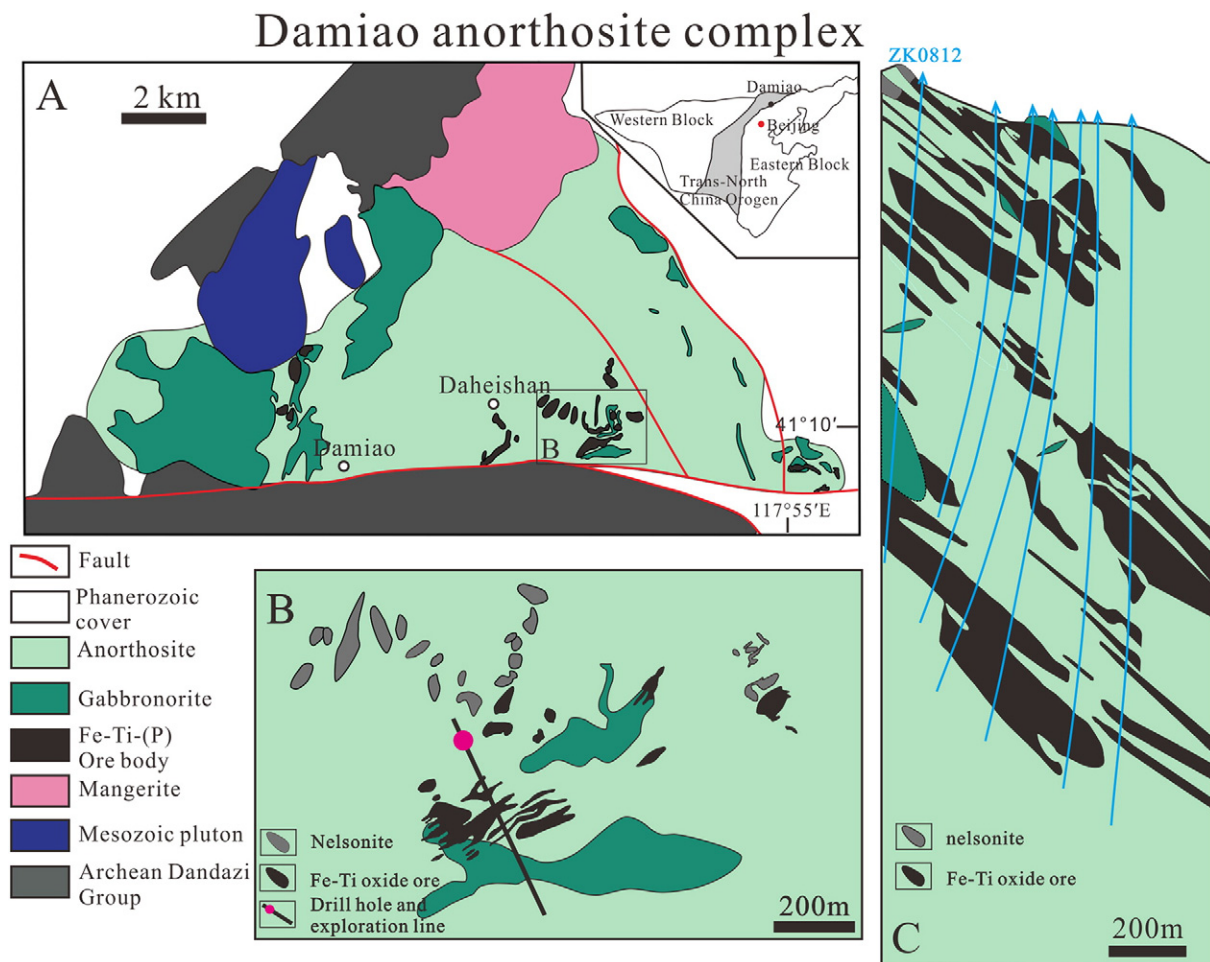
Fig. 1. A. Geologic map of the Damiao anorthosite complex; B. Lensoidal, irregularly-shaped veins of nelsonite and Fe–Ti oxides ore intruded into the anorthosite and gabbronorite; C. Cross section of the exploration line. Orebodies are lensoid or stratiform-like and situated (in the topographic lows) in the southern part of the anorthosite intrusion with various orientations, and wall rocks are anorthosite and gabbronorite (modified from the #4 Brigade of the Hebei BGMR, 2009).
