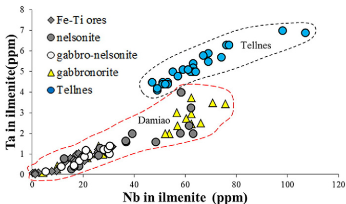
Fig. 12. Ilmenite from the various Damiao rock types contains a consistent Ta–Nb evolution trend.
