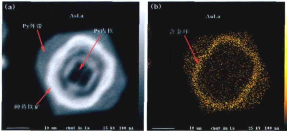
图 3 黔西南水银洞金矿床细粒黄铁矿的电子探针 X-ray 波谱 As(L \alpha )(a)和 Au(L \alpha )(b)成分扫描图像 Fig. 3 As La (a), Au La (b) composition scan image of pyrite through microprobe spectra scanning from Shuiyindong gold deposit in the southwestern Guizhou
