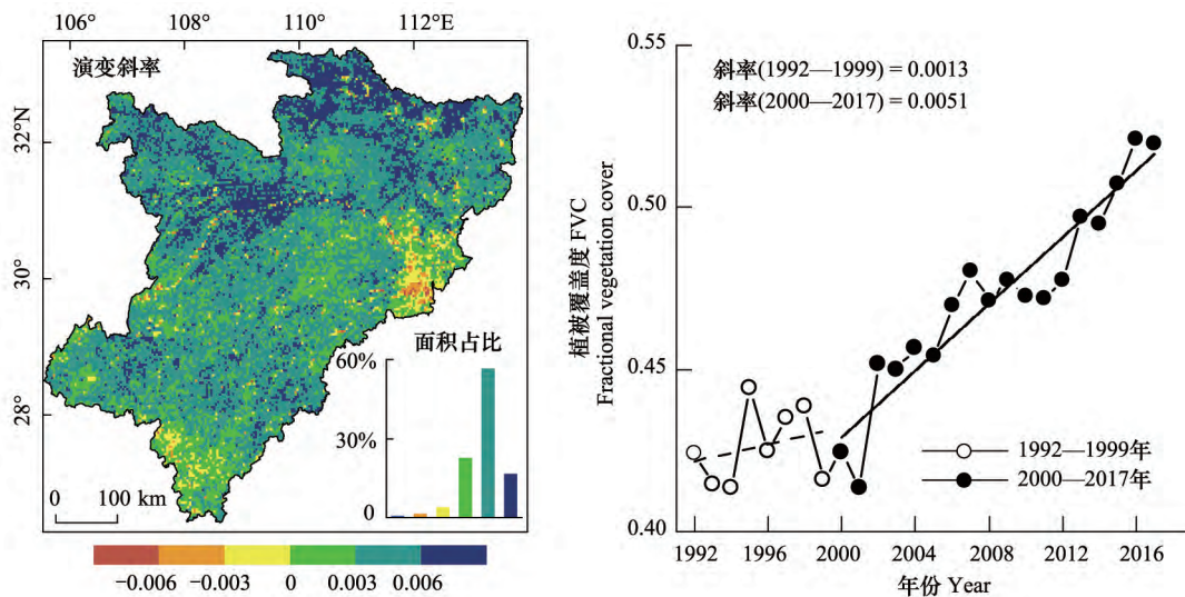
图4 槽谷年均FVC演变空间分布及整体演变趋势 Fig.4 Spatiotemporal variation of annual average FVC
