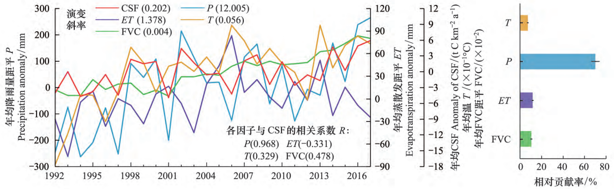
图8 槽谷喀斯特区域降雨(P)、温度(T)、蒸散发(ET)、植被覆盖度(FVC)和碳酸盐岩风化碳汇通量(CSF)的演变特征及各因子对碳酸盐岩风化碳汇通量(CSF)影响的相对贡献率 Fig.8 Temporal variations of annual average precipitation (P), temperature (T), evapotranspiration (ET), FVC and CSF with the relative contribution rates of factors to CSF
