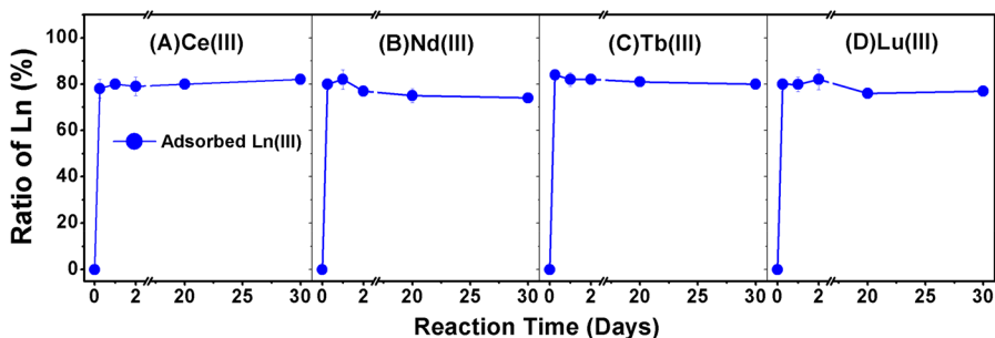
Figure 7. Temporal ratio changes of different Ln(III) species during adsorption on FHY: (A) Ce(III), (B) Nd(III), (C) Tb(III), and (D) Lu(III).
