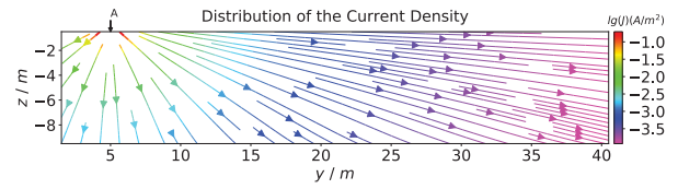
Figure 11. Uniform half-space current density distribution caused by a current point source.
