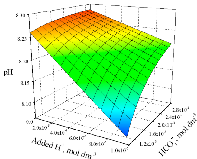
Figure 1. Equilibrium pH of seawater as a function of the concentrations of bicarbonate and added H^+ .
