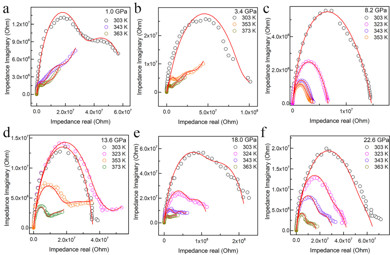
FIG. 1. AC impedance spectrum of SrCoO 2.5 at selected pressures and temperatures. Panels of (a), (b), (c), (d), (e), and (f) are the AC impedance spectrum at 1.0, 3.4, 8.2, 13.6, 18.0, and 22.6 GPa at temperatures between 303 and 373 K, respectively. The solid lines are the fitting results by the equivalent circuit.
