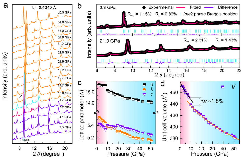
FIG. 3. Structural evolution of SrCoO 2.5 under high pressure probed by synchrotron x-ray diffraction. (a) Selected x-ray diffraction patterns at room temperature and high pressures. Incident x-ray wavelength is \lambda = 0.4340 \text{ \AA} . (b) Representative Rietveld refinement profiles at 2.3 and 21.9 GPa. (c) Lattice parameters vs pressure. (d) P - V equation of state up to 51 GPa.
