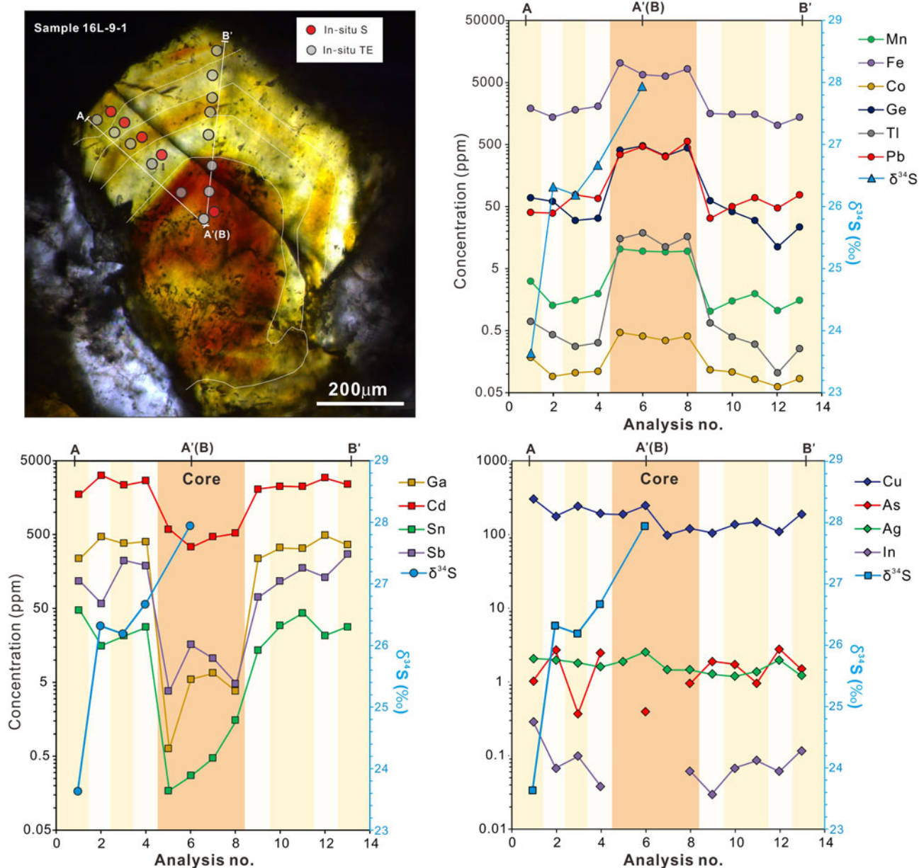
Fig. 7. Detailed traverses obtained for the CMR pattern of sphaerite from sample 16L-9-1 showing the variation of trace elements and sulfur isotopes in a sphaerite crystal. TE= trace elements.
