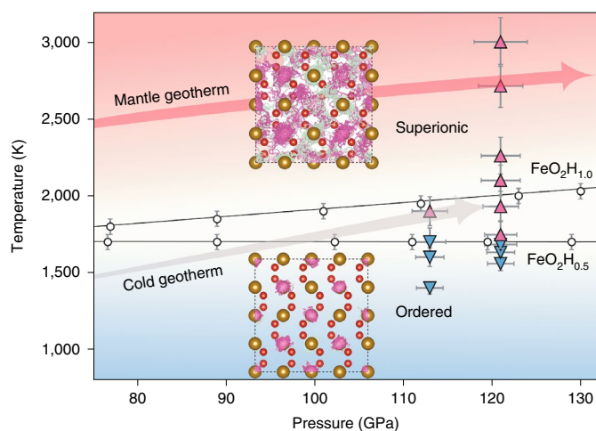
Fig. 1 | P-T phase diagram for ordered to superionic \text{FeO}_2\text{H}_x . Open circles are data points in the FPMD simulation. Error bars are statistic perturbations of T in each simulation. Uncertainty of P is within \pm 2 GPa. Upward and downward triangles represent the superionic and ordered phases, respectively, on the basis of EC measurements. Inset figures are the crystal lattice of \text{FeO}_2 with diffusive H (purple and green clouds represent different H layers).
