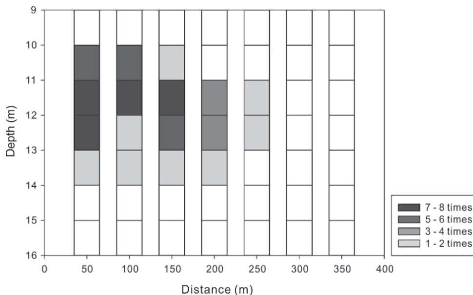
Fig. 3. Statistics of the monitoring results of the intrusion.
