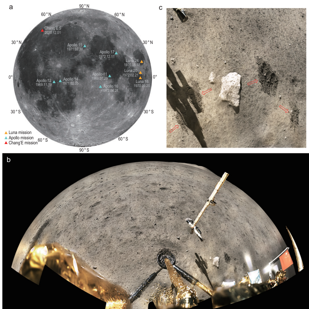
Figure 1. The distribution of lunar sampling sites and images of the CE-5 sampling site. (a) Lunar sampling sites and dates. Apollo and Luna sampling sites are within 30^\circ of low latitude. The CE-5 sampling site is in a new area at mid-latitude. The image data are from the CE-1 global digital orthophoto map (DOM). Detailed information about these sites can be found in Supplementary Table 1. (b) The panoramic image of the CE-5 landing site. The 120 images taken by the panoramic camera onboard the CE-5 lander were mosaiced using fisheye projection, with a horizontal field of view \sim 220^\circ . (c) A partial image of CE-5 scooped sampling. The arrows show the trace of scooped sampling. All images are from the China Lunar Exploration Data Release Website ( https://moon.bao.ac.cn ).
