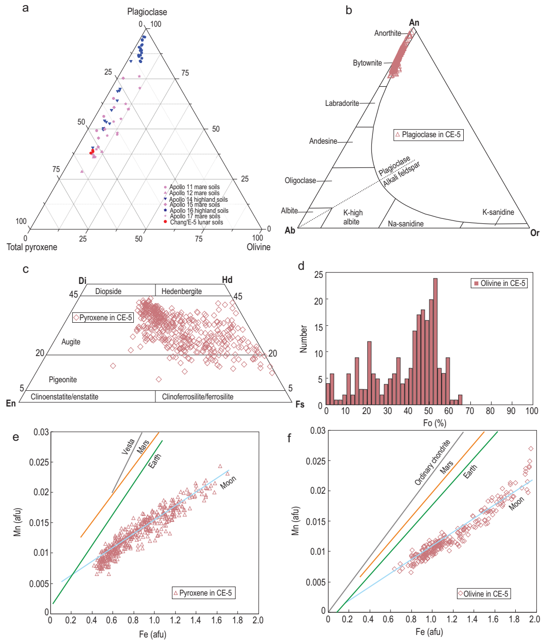
Figure 5. Mineral composition of CE-5 lunar soils compared with Apollo and Luna samples. (a) The triangular plot of major mineral abundances. CE-5 lunar soils are significantly enriched in pyroxene and low in olivine. The data of Apollo and Luna soils are from Refs [40,41]. (b)–(d) The mineral composition of plagioclase, pyroxene and olivine in CE-5 lunar soils. Plagioclase is mostly within the composition of bytownite. Pyroxene lies within the range of high-calcium pyroxene and is dominated by augite with a small amount of pigeonite. Olivine is mostly fayalite. (e), (f) Mn versus Fe atoms per formula unit in pyroxene and olivine in CE-5 lunar soils. Planetary trend lines are from Ref. [32] and references therein. Abbreviations: afu, atoms per formula unit.
