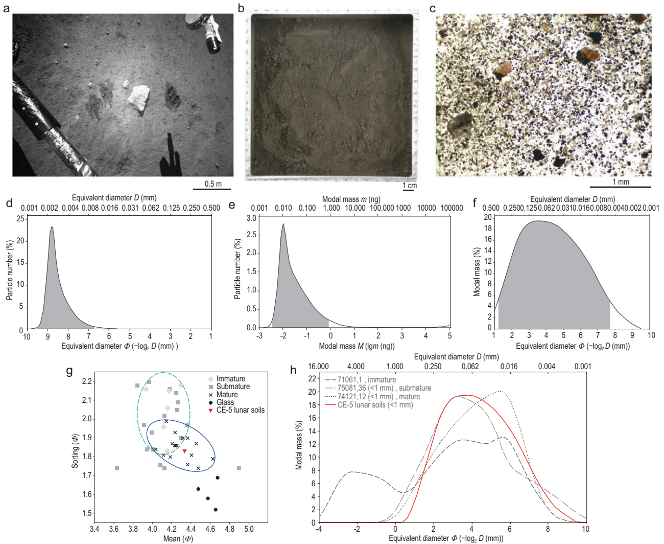
Figure 3. Image characteristics and particle size distribution of CE-5 lunar soils. (a) The surveillance camera image shows the characteristics of the lunar regolith at the sample site. The lunar regolith was mostly gray-black. The dark traces are the imprints after sampling. (b) A laboratory camera photo of scooped lunar regolith. (c) An image of lunar soil particles when magnified equivalent to the lunar soil grain size using a stereomicroscope (e.g. yellow-green olivine, white feldspar, brown-black pyroxene and brown glass). (d) The number (percent) distribution of particle size (equivalent diameter). Particle sizes range from 1.11 \mu\text{m} to 499.8 \mu\text{m} , with a mean of 3.96 \mu\text{m} , a median of 2.90 \mu\text{m} and a mode of 3.39 \mu\text{m} . Of the particles, 95% (the gray part) are distributed between 1.40 \mu\text{m} and 9.35 \mu\text{m} . (e) The modal mass (percent) distribution of particle size. The modal mass ranges from 0.0012 ng to 109177.8937 ng, with a mean of 0.5567 ng, a median of 0.0205 ng and a mode of 0.0095 ng. Of the particle mass, 95% (the gray part) is distributed between 0.0036 ng and 0.8304 ng. (f) The modal mass-grain size distribution of CE-5 lunar soils. Of the particle mass, 95% (the gray part) is distributed between 4.84 \mu\text{m} ( \Phi 7.69) and 432.27 \mu\text{m} ( \Phi 1.21), with a mean of 49.80 \mu\text{m} ( \Phi 4.33), a mode of 88.38 \mu\text{m} ( \Phi 3.50) and a median ( \Phi_{50} ) of 52.54 \mu\text{m} ( \Phi 4.25). (g) The grain size-sorting comparison between CE-5 and Apollo 17 lunar soils. CE-5 lunar soils tend to be mature. Apollo 17 lunar soil data are from Ref. [33]. (h) The comparison of modal mass-grain size distribution between CE-5 and Apollo lunar soils of varying maturity. The red solid line is CE-5 lunar soils, the dashed line is Apollo 17 (71061,1) immature lunar soils, the dot-dashed line is Apollo 17 (75081,36) submature lunar soils and the dotted line is Apollo 17 (74121,12) mature lunar soils. Apollo 17 lunar soil data are from Ref. [33].
