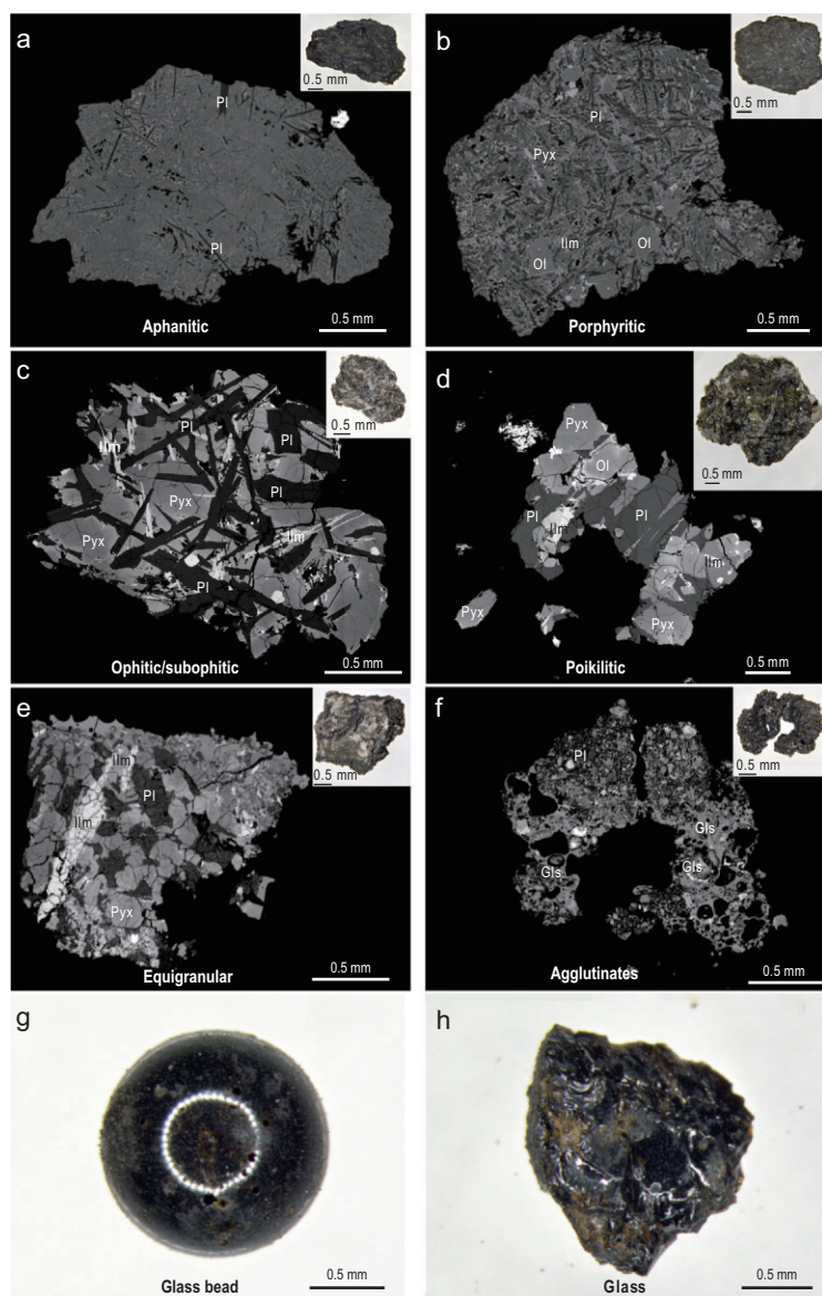
Figure 4. BSE images and stereomicrographs of typical basaltic clasts, agglutinate and glasses from the CE-5 lunar sample. (a)–(f) BSE images for basaltic clasts and agglutinate with different textures. The upper right corner of the BSE image is the stereomicrograph corresponding to each clast. (g), (h) Stereomicrographs of glass. Abbreviations: Pyx, pyroxene; Pl, plagioclase; Ol, olivine; Ilm, ilmenite; Glass, Gls.
