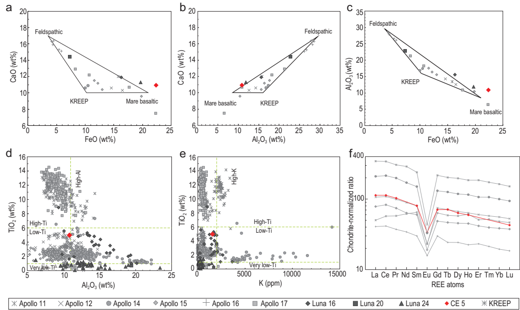
Figure 6. The chemical composition of CE-5 lunar soils compared with Apollo and Luna collections. (a)–(c) Elemental variations of Al 2 O 3 , CaO and FeO (database and triangles from Ref. [16]). (d), (e) TiO 2 , Al 2 O 3 and K classification scheme of mare basalts. The protoliths of CE-5 lunar soils belong to the low-Ti/low-Al/low-K species (database from Ref. [4]). (f) Chondrite-normalized concentrations of REE in lunar soils as a function of an REE atom. The REE pattern of CE-5 lunar soils shows negative Eu anomalies. The database of Apollo samples is from Ref. [16] and the KREEP composition data are from Ref. [46]. Normalization values: 1.36C, where C represents the ‘Mean C1 Chondr.’ values of Table 1 in Ref. [48].
