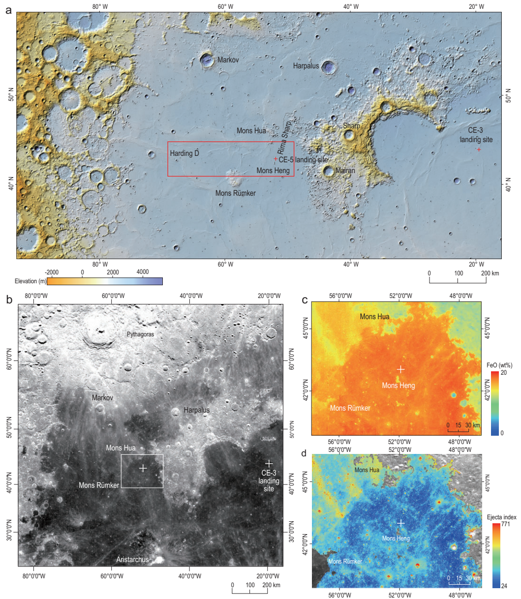
Figure 2. Geographical and geological backgrounds of the CE-5 lunar sample. The ‘+’ in all images are CE landing sites. (a) Topographic map with the red box showing the selected landing area. The topographic data are from the CE-2 global digital elevation model data. (b) Image and geological background of the landing site with the ejecta distribution. The white box is the area of c and d. Image data are from CE-2 global DOM. (c) Spectral concentration map of FeO (wt%) in the sampling area. It shows that the sampling site is uncontaminated by ejecta materials. FeO content is derived from https://astrogeology.usgs.gov/search/map/Moon/Kaguya/MI/MineralMaps/Lunar Kaguya MI/Map MineralDeconv FeOWeightPercent 50N50S . (d) The enlarged map of the relative ejecta concentration index of the sampling area. The sampling site is free of ejecta contamination. All CE images are from the China Lunar Exploration Data Release Website ( https://moon.bao.ac.cn ).
