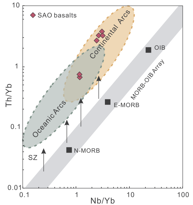
Fig. 14. Nb/Yb-Th/Yb diagram for the SAO basalts (modified after Pearce, 2014).
