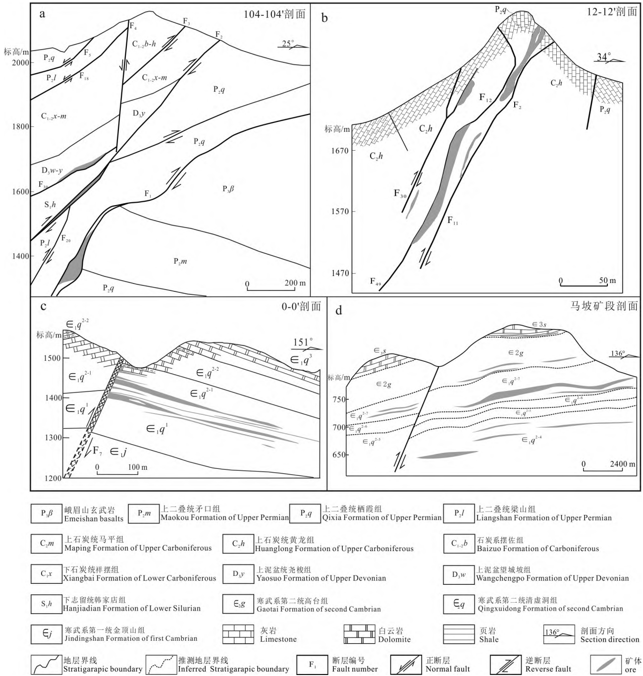
图2 典型矿床剖面图(据金中国等,2020) a. 猪拱塘矿床; b. 杉树林矿床; c. 那雍枝矿床; d. 牛角塘矿床 Fig. 2 Geological sections of typical ore deposits (after Jin et al., 2020) a. Zhugongtang deposit; b. Shanshulin deposit; c. Nayongzhi deposit; d. Niujiaotang deposit
