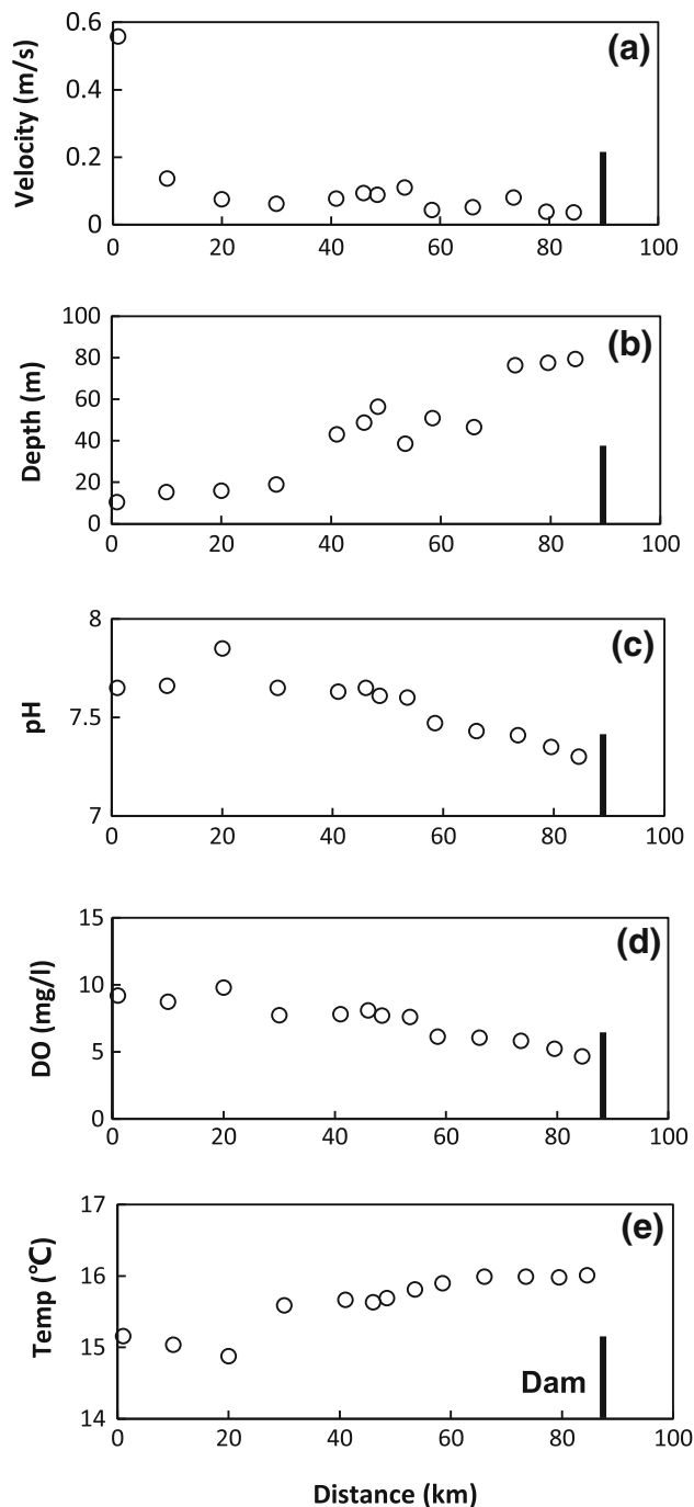
Fig. 3 Variation of velocity, depth, pH, Temp, DO along the Wujiangdu Reservoir
