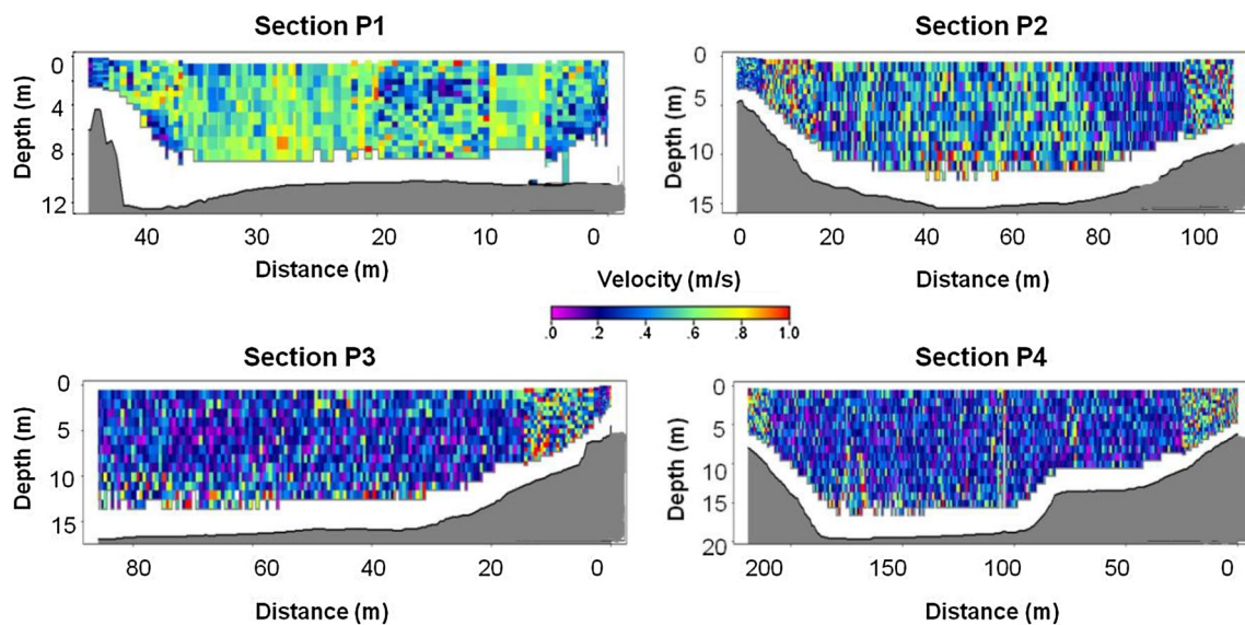
Fig. 4 The velocity variation of sections
