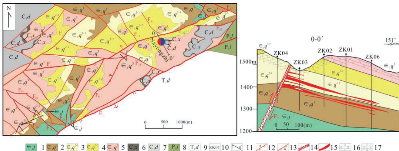
Fig.1 Geological map and No.0 cross section of the Nayongzhi Pb-Zn deposit 1-Lower Cambrian Jindingshan Formation; 2-First section of the Lower Cambrian Qingxudong Formation; 3-First layer of the second section of the lower Cambrian Qingxudong Formation; 4-Second layer of second section of the lower Cambrian Qingxudong Formation; 5-Third section of the lower Cambrian Qingxudong Formation; 6-Lower Carboniferous Xiangbai Formation; 7-Lower Carboniferous Dapu Formation; 8-Upper Permian Longtan Formation; 9-Lower Triassic Daye Formation; 10-Drill and number; 11-Cross section and number; 12-Thrust fault; 13-Nomal fault; 14-Steep veined ore body; 15-Stratiform ore body; 16-Dolomite; 17-Argillaceous dolomite
