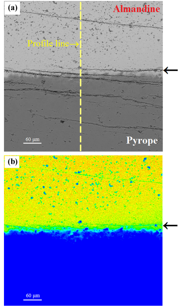
Fig. 3. (a) Backscattered electron image of a garnet diffusion couple (Z018-b). The experiment was annealed at 3 GPa and 1473 K for 24 h under wet condition ( \sim 531 weight ppm \text{H}_2\text{O} ). The interface between the two halves of the diffusion couple is indicated by arrow. The position of one of the measured compositional profiles is indicated by a yellow dashed line; this direction is perpendicular to the interface. (b) Element map of Fe in wet diffusion couple of (a). The iron content decreases from yellow area (almandine) at the top of the image to blue area (pyrope) at the bottom. Note that, a marked diffusion zone can be clearly seen close to the initial interface. (For interpretation of the colors in Fig. 3, the reader is referred to the web version of this article.)
